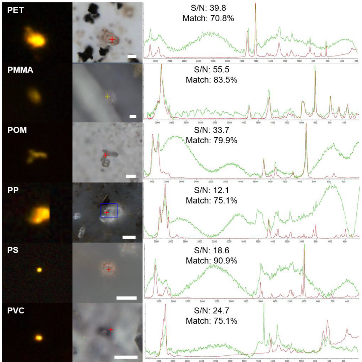
Figure 4. Examples of MP particles found in human tissue samples displayed as fluorescence images (left column) and true color microscope images (mid column) as well as related Raman-spectra. White scale bar indicates 10 \mu\text{m} , library reference spectra are displayed in red, particle spectra are given in green. S/N: signal to noise ratio.
