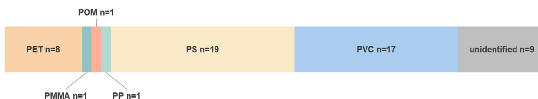
Figure 3. Polymeric composition of particles found in human tissue samples ( n = 56).
