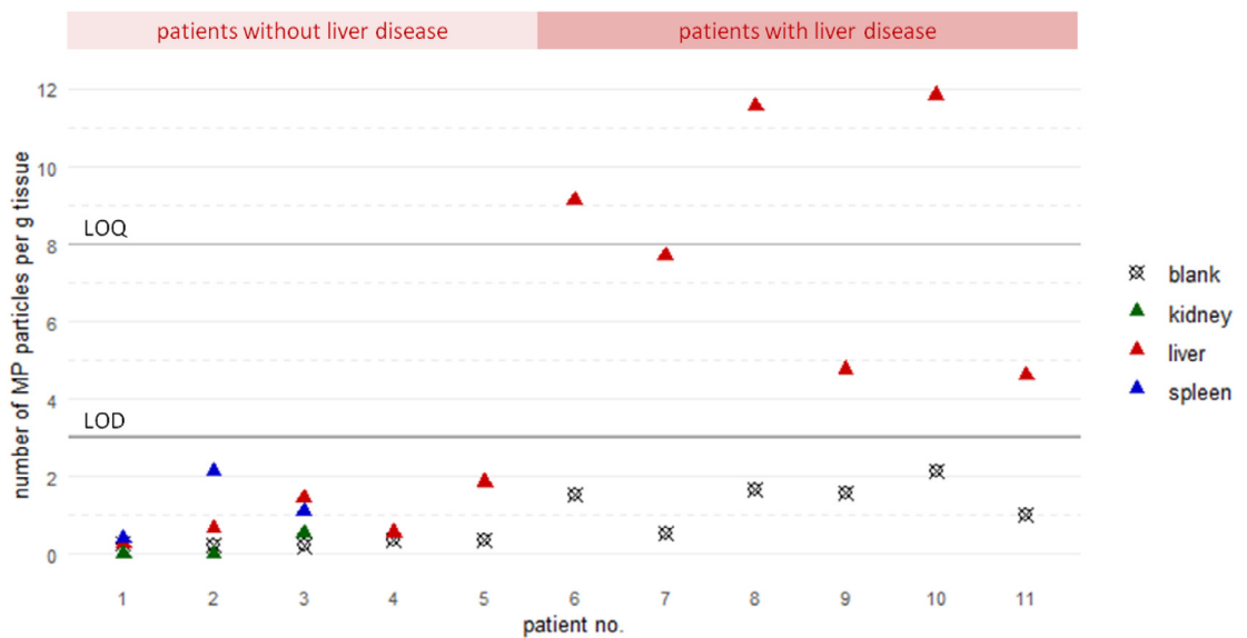
Figure 2. MP concentrations per patient, organ and associated blank (number per weight of tissue). Limit of Detection LOD = 3.0282 (mean + 3*SD); Limit of Quantification QOD = 7.9982 (mean + 10*SD).
